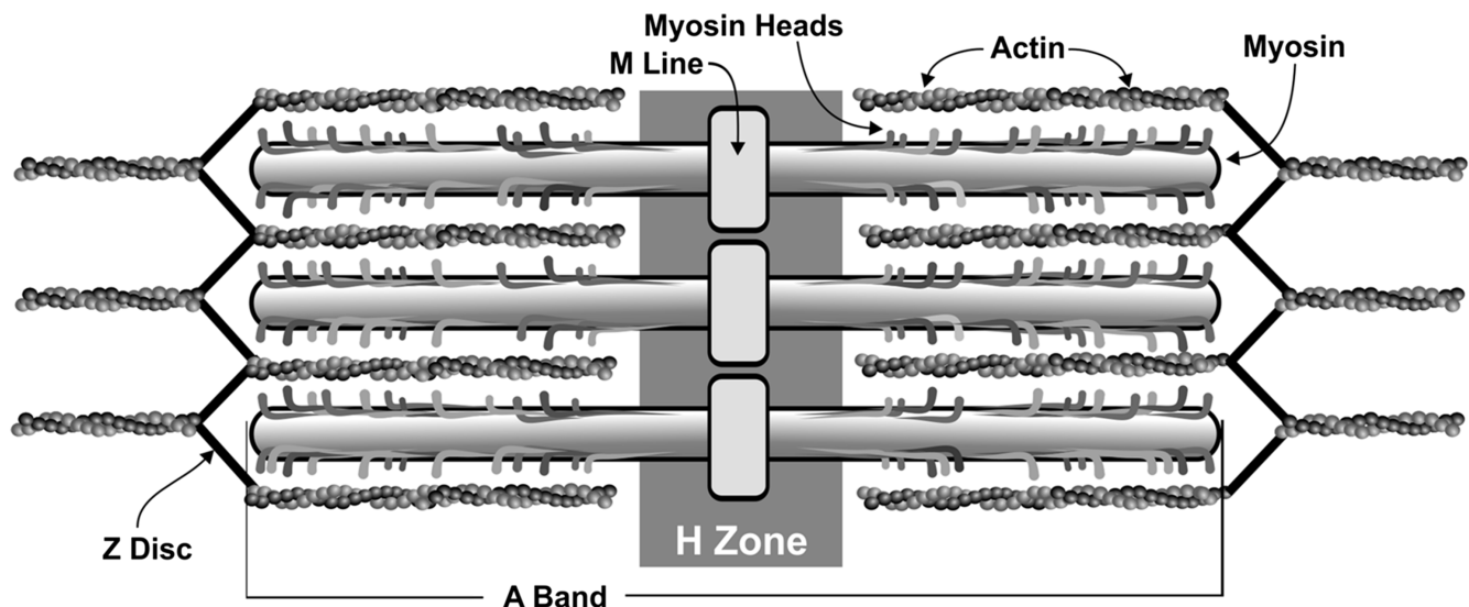
Figure 1. Sarcomere organization. A sarcomere is the smallest functional unit of muscle contraction. It is organized from Z disc to Z disc (termed the A Band), with an M line found in the center. The functional unit consists of the actin and myosin filaments, which will slide over one another toward the M line during contraction and shrink the H zone. Image reprinted with permission of John Nagy.
